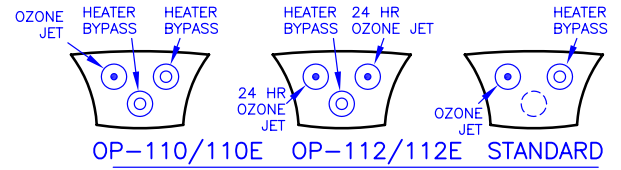
VIEW A
