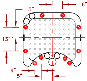
AIR INJECTORS LOCATION
